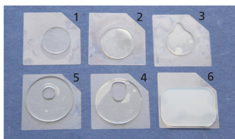
Regensensorpads
